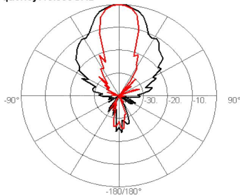
Frequency:18.000GHz
