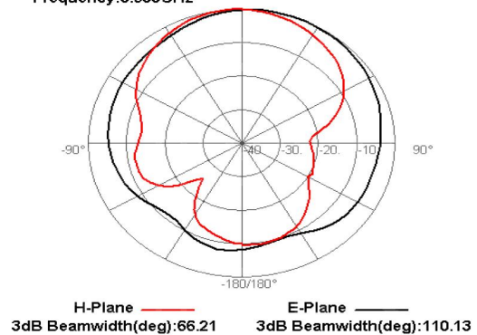
Frequency:0.600GHz
