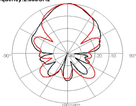
Frequency:2.000GHz
