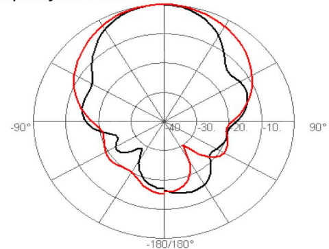
Frequency:0.800GHz
