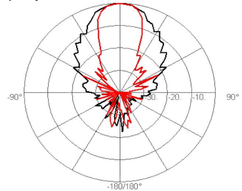
Frequency:12.000GHz
