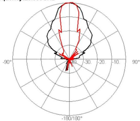
Frequency:26.000GHz
