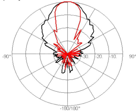
Frequency:14.000GHz
