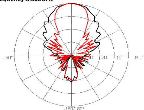
Frequency:9.000GHz
