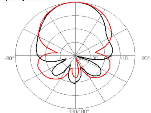
Frequency:1.000GHz
