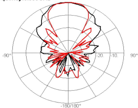
Frequency:6.000GHz
