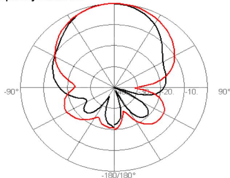
Frequency:0.900GHz
